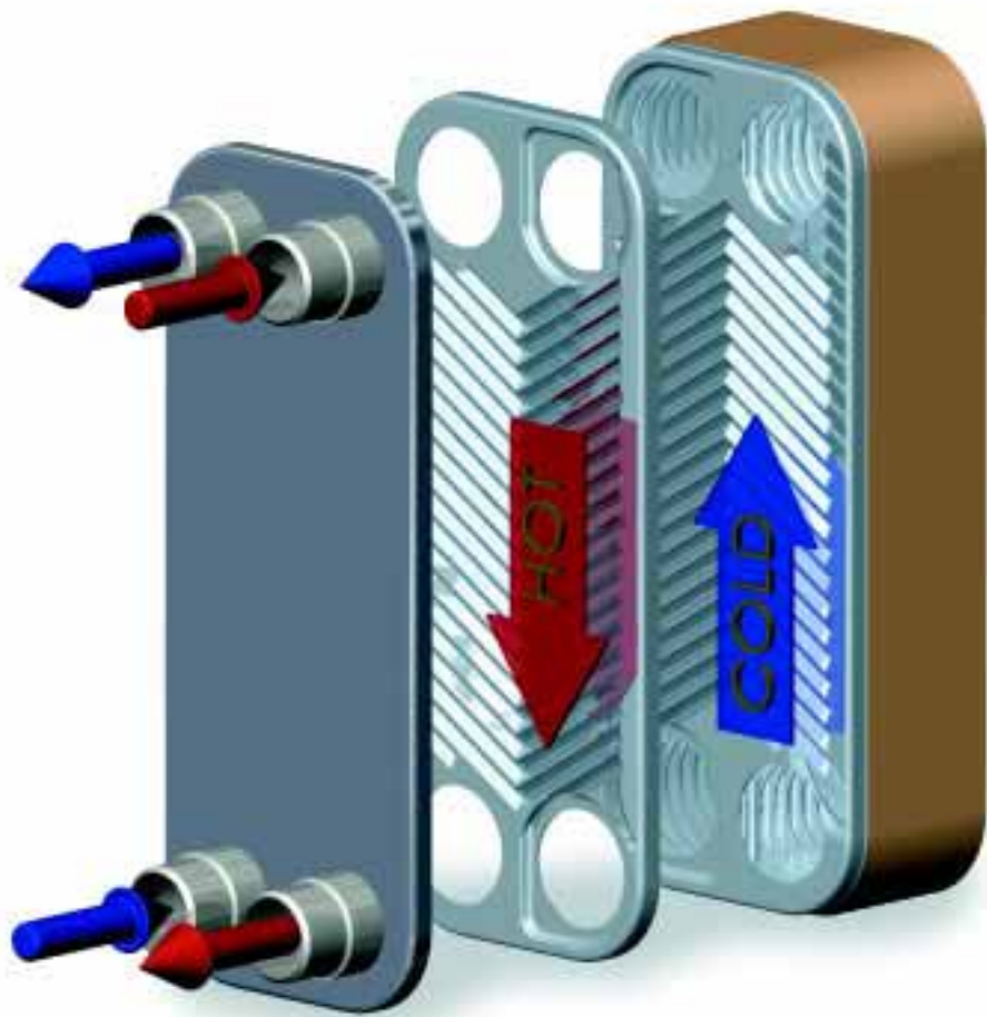
Exploded view of API Schmidt-Bretten SB Braze Plate Heat Exchanger.
