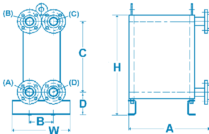
General dimensions Not for construction purposes
